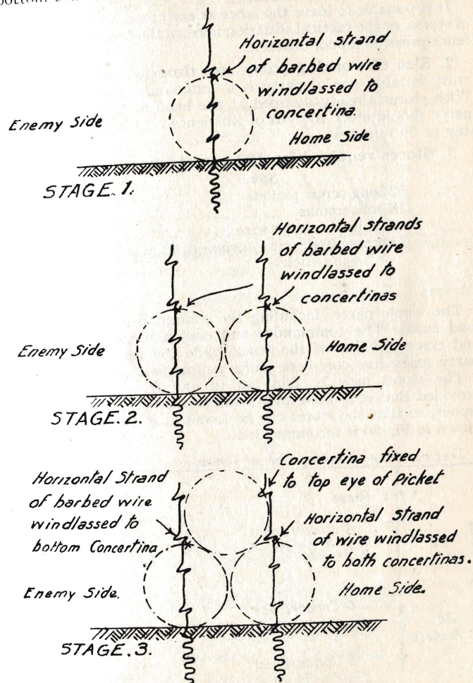
FIG 29.—TRIPLE CONCERTINA FENCE
