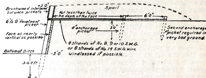
FIG 24.—TANK DITCH REVETMENT
