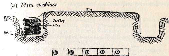
FIG 17.—ANTI-TANK MINE NECKLACE
