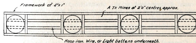
FIG 18.—ANTI-TANK MINE SLED
