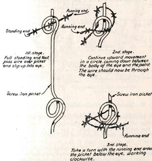
FIG 26.—METHOD OF FIXING WIRE TO PICKETS TOP EYE
