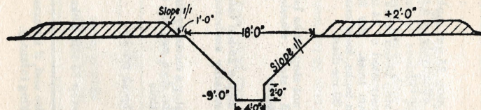
FIG 4.—V TANK DITCH
