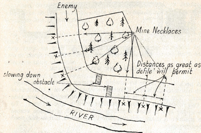
FIG 19.—NECKLACE OR SLED ROAD BLOCK
