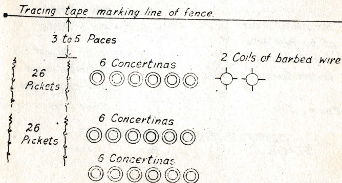
LAYOUT OF STORES FOR 100 YDS TRIPLE CONCERTINA FENCE
