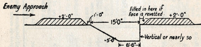
FIG 5.—"ONE-WAY" TANK DITCH
