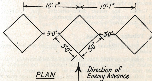
FIG 7.—REINFORCED CONCRETE CUBES
