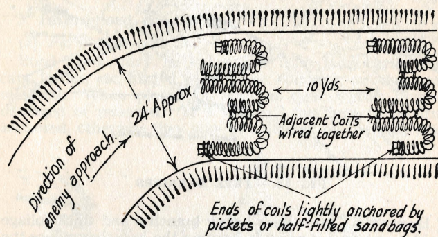
FIG 16.—CONCERTINA ROAD BLOCK
