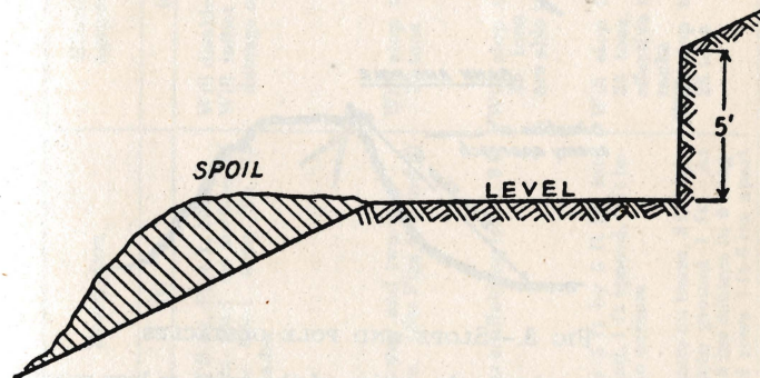
FIG 2.—SCARPED SLOPE .
