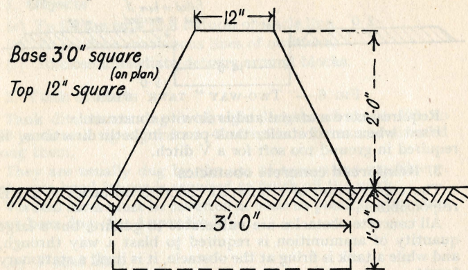
FIG 8.—REINFORCED CONCRETE "PIMPLE"
