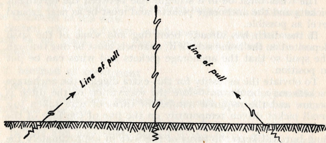
FIG 25.—ANCHOR PICKETS
