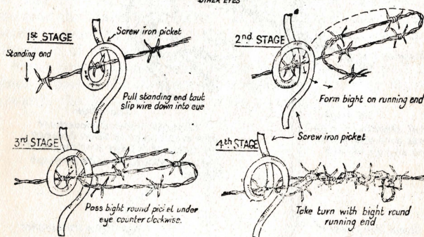
FIG 27—METHOD OF FIXING WIRE TO PICKETS OTHER EYES
