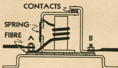
Fig. 1—The buzzer type circuit breaker.
