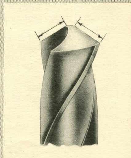
Fig. 6. Each cutting edge must be the same length in order to split the work evenly and make the right size hole.
