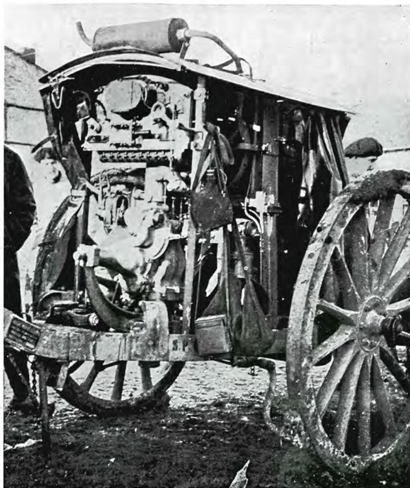
A FRENCH VERDUN SEARCHLIGHT: INTERIOR OF AN ELECTRICITY-GENERATING VAN. The mobile van which contains the electricity-generating mechanism and intricate installation of engine-apparatus required for one of the types of searchlights in use by the French at Verdun and elsewhere, is seen in detail above. For the exhibition of the complex interior the ends and sides of the vehicle are shown open.—[French Official Photograph; supplied by Newspaper Illustrations.]
